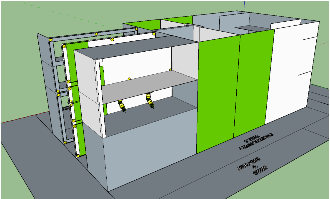
Figure 10.2b — Storage and shelving elevation with robot-arm cells, and the shelving-to-printer aisle.
