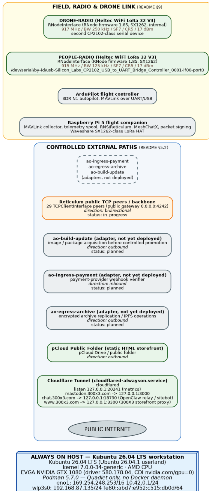
Figure 3.1.1d — Field, radio, and controlled external paths (Sections 9 and 11)
